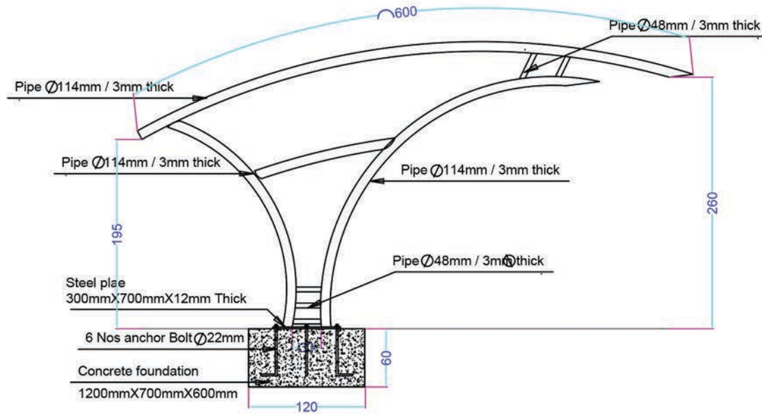
Side - SECTION
